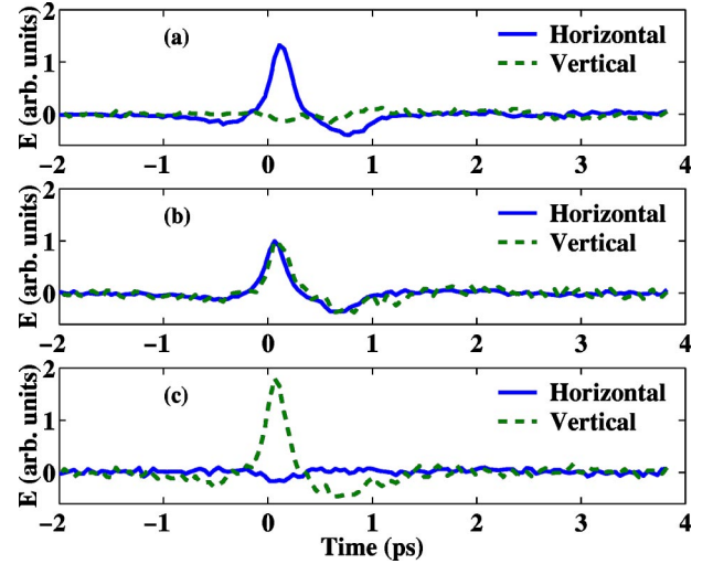
FIG. 2. (Color online) Horizontal (solid) and vertical (dashed) components of THz electric field (obtained from measured voltage) are plotted against time with the emitter at (a) 0^\circ , (b) 45^\circ , and (c) 90^\circ , respectively.
