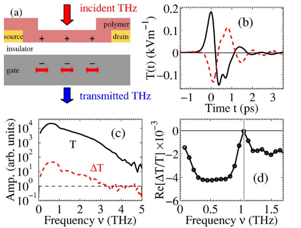
FIG. 1. (Color online) (a) Schematic diagram of the transistor sample geometry for terahertz TDS. Application of a negative gate voltage gives rise to holes in the accumulation layer in the polymer and highly mobile electrons in the silicon gate. (b) Measured terahertz electric field T(t) after transmission through transistor (solid line) and change in transmitted terahertz electric field \Delta T(t) (dashed line, multiplied by 100) upon application of a gate voltage V_g=0 \leftrightarrow -30 V. Both are given as a function of electro-optic sampling delay time t . (c) Amplitude spectra of the transmitted radiation T(\nu) , and change in transmitted amplitude \Delta T(\nu)=T(V_g=-30 \text{ V})-T(V_g=0 \text{ V}) obtained from the time-domain data in (b) through Fourier transformation. (d) Change in transmission \Delta T/T as a function of frequency. The artefact close to 1 THz is a result of diffraction from the interdigitated array formed by the electrodes, as explained in the text.
