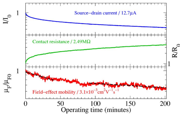
FIG. 3. (Color online) Source current (top), source contact resistance (middle), and field-effect mobility \mu_F (bottom) of a 2 \mu\text{m} channel length F8T2/300 nm \text{SiO}_2/\text{Si} pFET as a function of operating time, normalized to their initial values, and shown on a semilogarithmic plot. The curves were extracted from scanning Kelvin-probe microscopy measurements across the transistor channel. A constant gate voltage bias of V_g = -40 \text{ V} was applied to produce an initial sheet charge density n_h = 2.9 \times 10^{12} \text{ cm}^{-2} comparable to that in the terahertz experiments. The dotted lines are exponential fits to \mu_F at early and late operating times, with time constants \tau = 1.2 \times 10^4 \text{ s} and \tau = 5.6 \times 10^4 \text{ s} , respectively.
