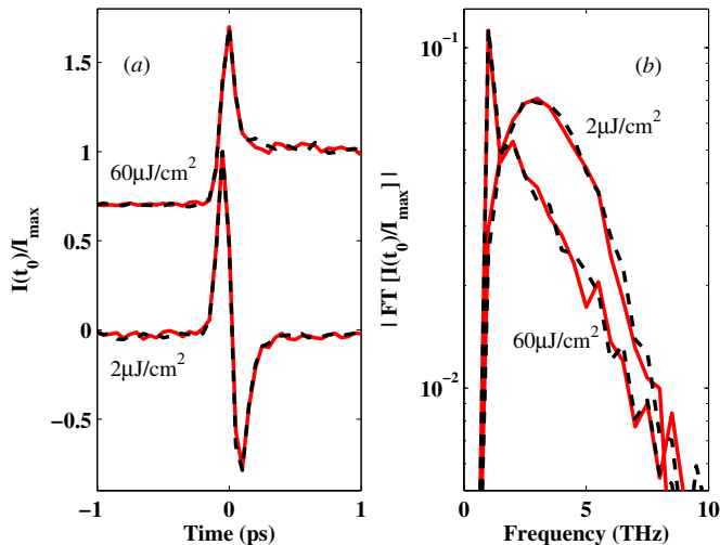
Figure 5. (a) Normalized current simulated as a function of relative delay between the optical gate pulse and THz transient. The curves show the simulations for gate fluences 2 and 60 \mu\text{J cm}^{-2} with (continuous) and without (dashed) carrier–carrier scattering for a GaAs photoconductive detector with a trap density of 2 \times 10^{18} \text{ cm}^{-3} . (b) The Fourier transform of the curves in (a). There is a negligible variation between the curves with and without the scattering mechanism.
