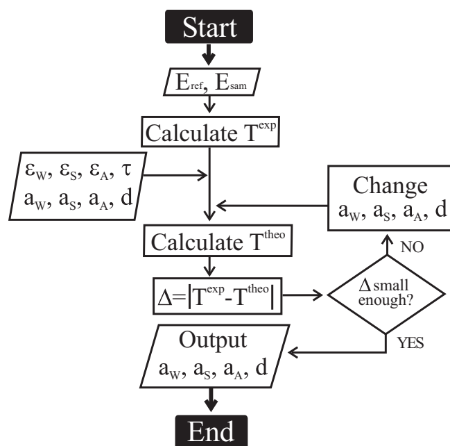
Figure 2. (Color online) Flow chart of iterative algorithm used to determine the volumetric fraction of water in a leaf. The algorithm calculates the experimental transmission function and compares it to a theoretical transmission coefficient calculated from the combination of the dielectric functions of its components according to the model presented.
