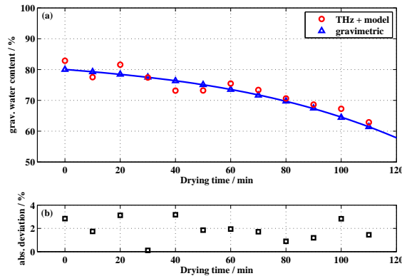
Figure 4. (Color online) Terahertz-based (circles calculated with Eq. 5) and gravimetric (triangles calculated with Eq. 6) quantification of weight-percentage of water contents in leaves. At t = 0 the leaves were separated from a live plant and they were maintained in an oven at 60^{\circ}\text{C} between measurements in order to accelerate their dehydration. The continuous line is supplied as a "guide to the eye" and does not represent any actual measurement. The lower panel shows the absolute deviation between the terahertz and the gravimetric measurements.
