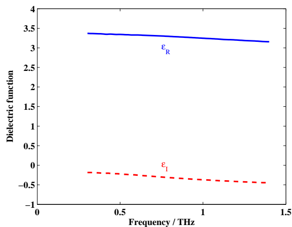
Figure 3. (Color online) Real (continuous) and imaginary (dashed) parts of the dielectric function of dry compact tissue measured by THz-TDS.
